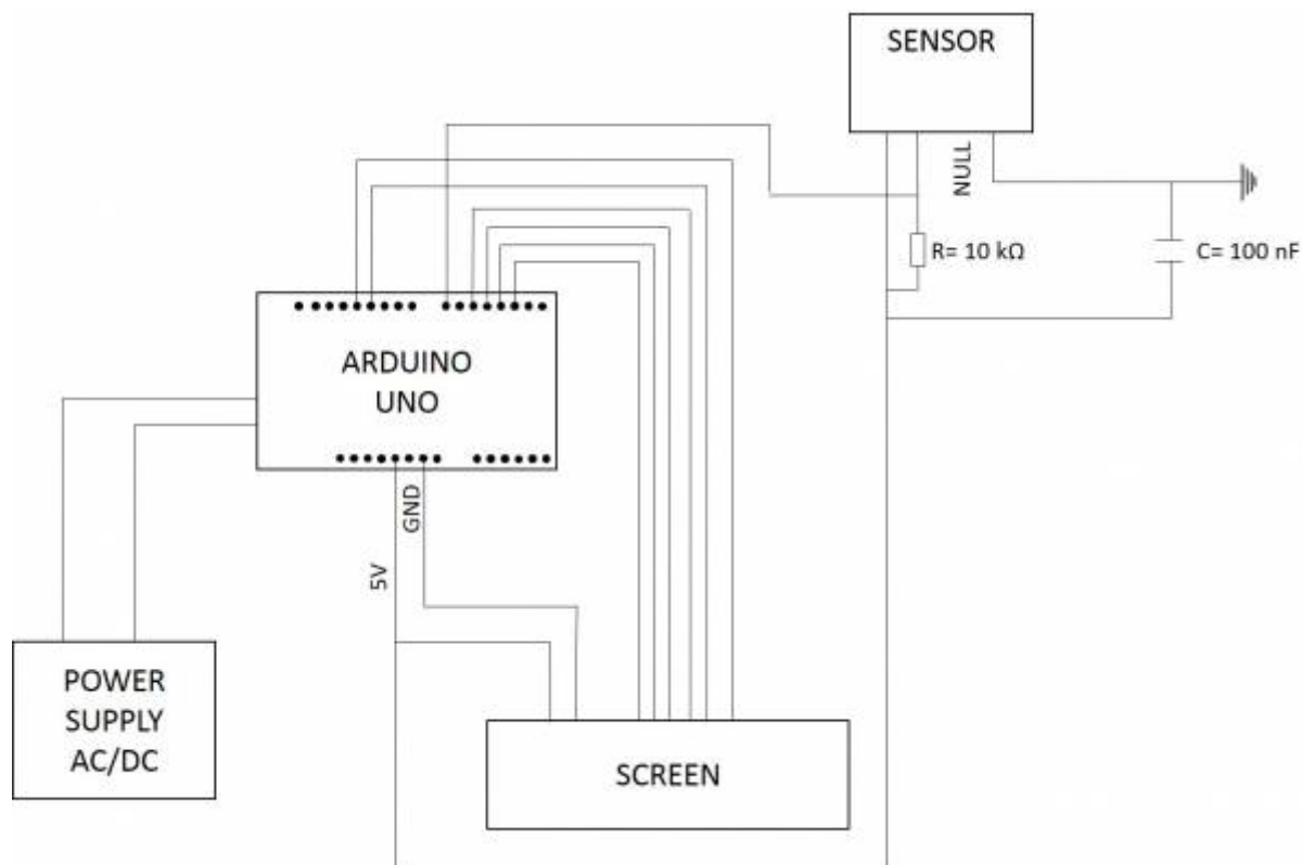
Figure 36: Electronic schematic
