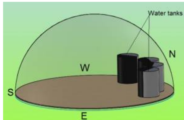
Figure 47: Heating system
