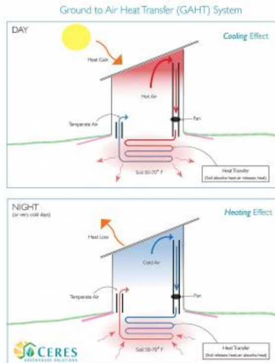
Figure 4: Figure 4. GAHT scheme
